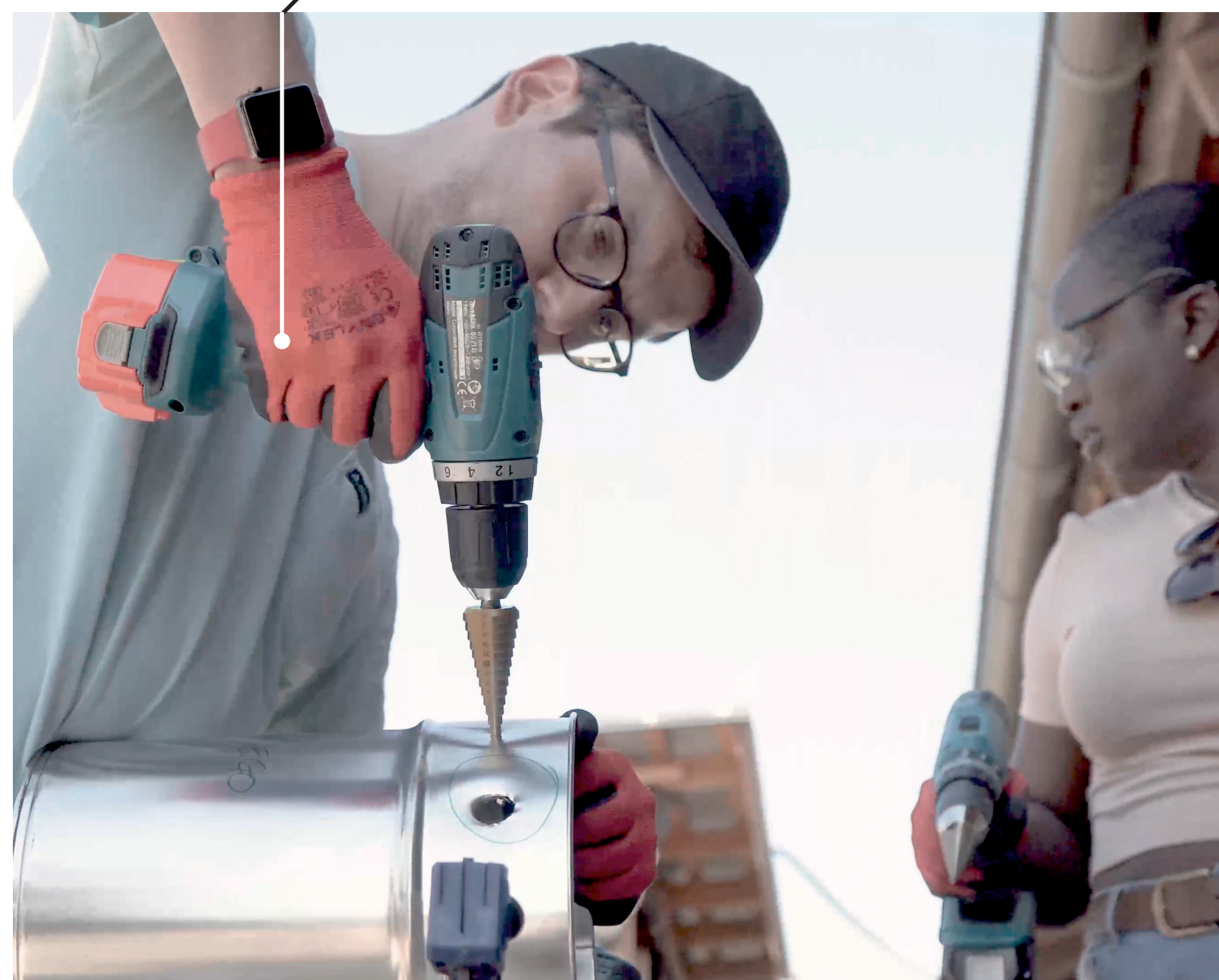
Upcycling cans into TLUD stove
